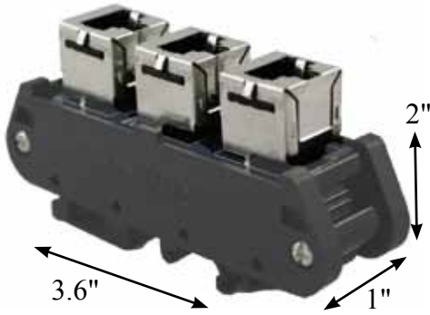
Type: IMRJ0845-1x3
