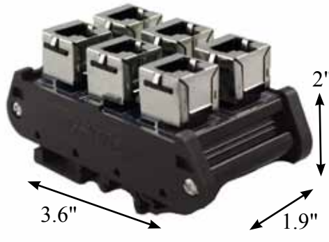
Type: IMRJ0845-2x3
