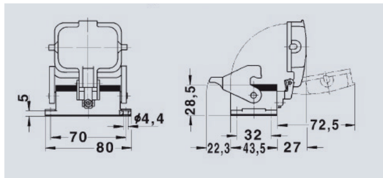
Housing Dimensions (mm)
