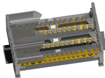
Upper view of the terminal board with cut-away protection cover
