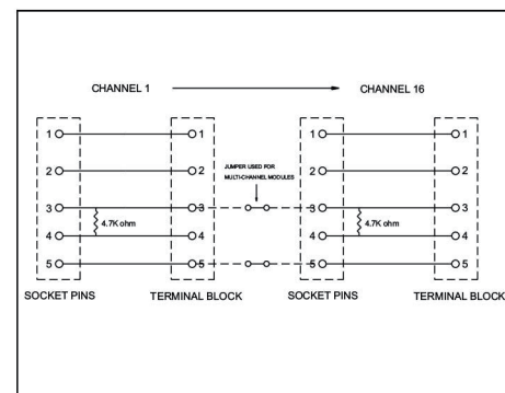
IMSR TYPICAL SCHEMATIC
